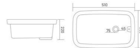
LAB SINK 20" x 15" x 8"
