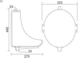
FLAT BACK Urinal 13" x 11" x 18"
