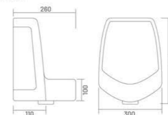
CORNER URINAL Urinal 12" x 10" x 14"
