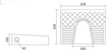
SQUATTING Urinal 17" x 13" x 4"
