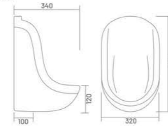
NANO LARGE Urinal 13" x 13" x 17"
